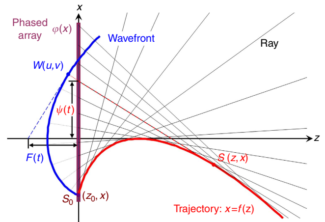
Figure 6 | Asymptotic theory of self-bending acoustic beams. The rays (thin black lines) emitted from the wavefront (blue curve) construct a caustic (red curve), creating a self-bending acoustic beam. Each ray is being a tangent of the trajectory. The phase modulation of the phased array (thick magenta line) is directly derived from the wavefront.
