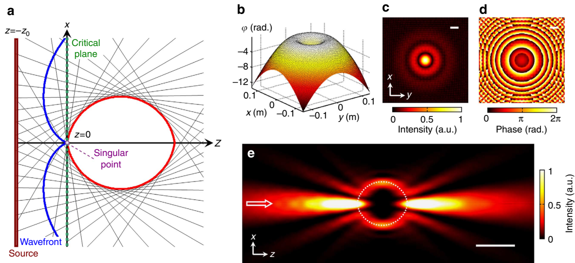
Figure 8 | Design methodology of acoustic bottle beams. (a) Illustration of the method. (b–e) Numerical simulation results. As shown in a , from the one-to-one mapping between the rays (thin black lines) and the boundary of the bottle beam (red curve) at the critical plane ( z = 0 , except the singular point), we first construct the wavefront (blue curve) and then the pure phase map ( b ) at the critical plane (vertical dashed line). With a backward propagating process, we can obtain the amplitude ( c ) and phase modulation ( d ) required for the production of the designed bottle beam at z = -z_0 , the intensity cross-section of which is shown in e , where the white dashed curves depict the predesigned bottle shape. Scale bar, 0.1 m. a.u., arbitrary unit.
