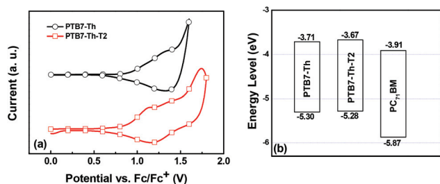
Fig. 3 Cyclic voltammograms of the oxidation curves (a) and HOMO and LUMO energy level diagrams of PTB7-Th-T2, PTB7-Th and PC 71 BM 45 (b).
