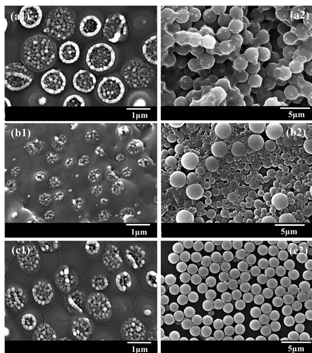
Fig. 3 SEM images of SAN particles (St : AN = 30 : 70 wt%) with different weight ratios of AIBN to BPO: (a1 and a2) 1.4 : 0, (b1 and b2) 0 : 1.4 and (c1 and c2) 0.8 : 0.6 (the left column, 0.5 h; the right column, final products).
